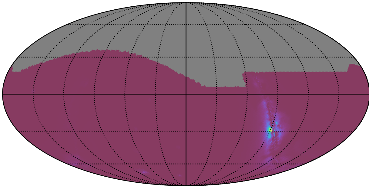
too_elab_heavy_r64_d3_ugrizy_v3.4_10yrs : NlcPoints
