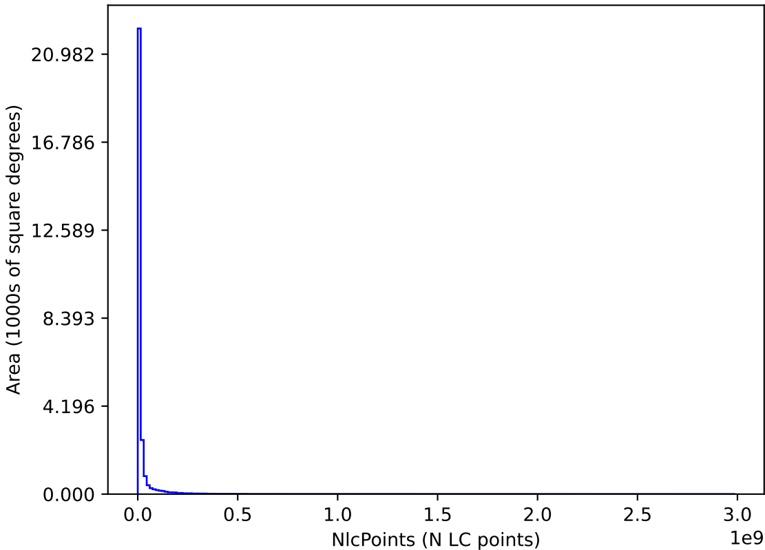
too_elab_heavy_r64_d3_ugrizy_v3.4_10yrs : NlcPoints
