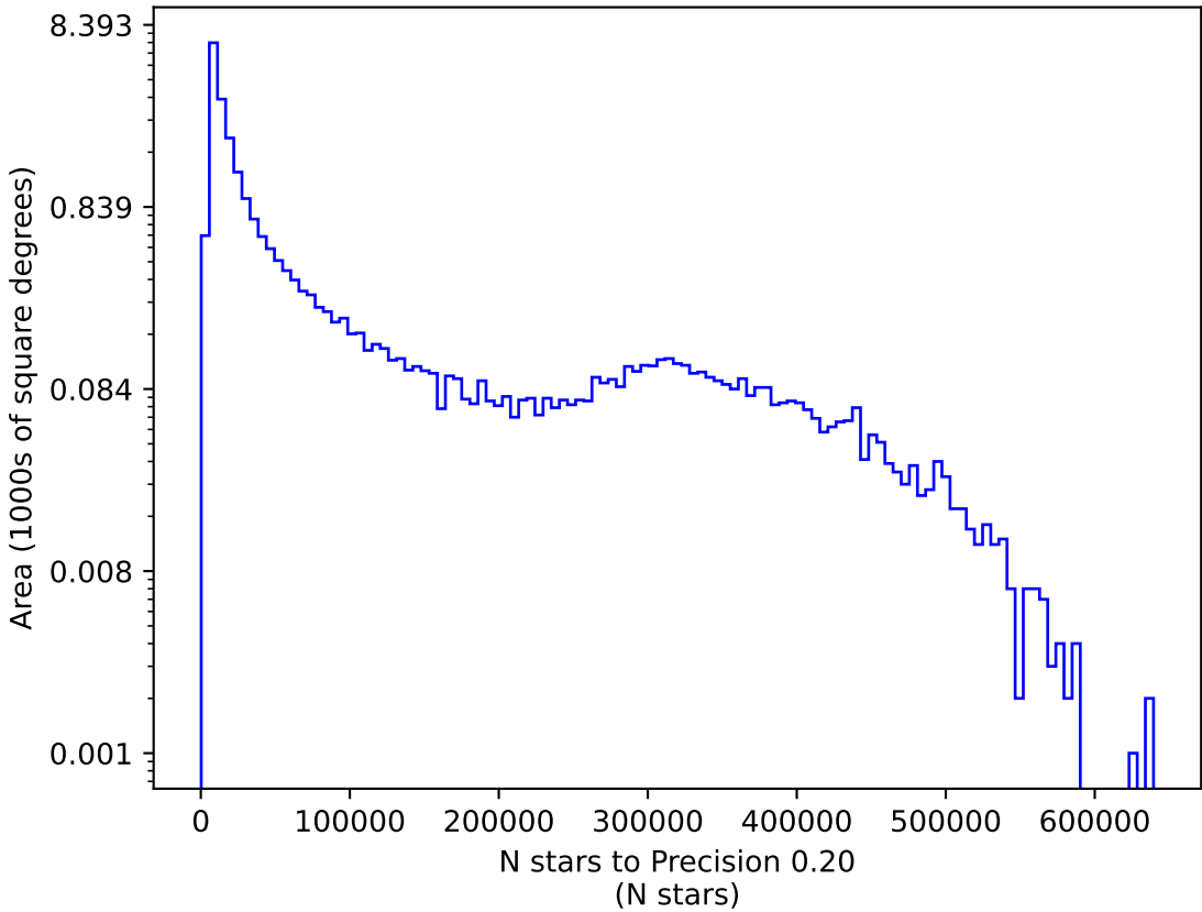
too_elab_heavy_r64_d3_ugrizy_v3.4_10yrs y: N stars to Precision 0.20
