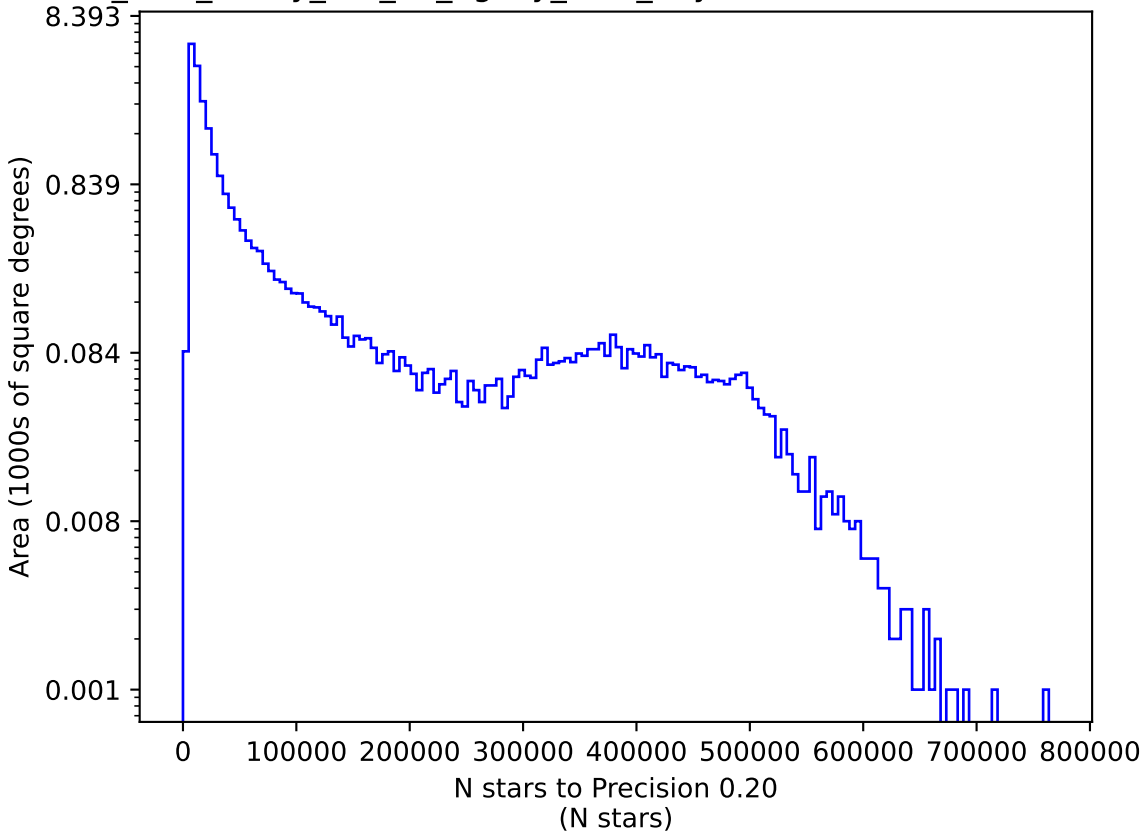
too_elab_heavy_r64_d3_ugrizy_v3.4_10yrs i: N stars to Precision 0.20
