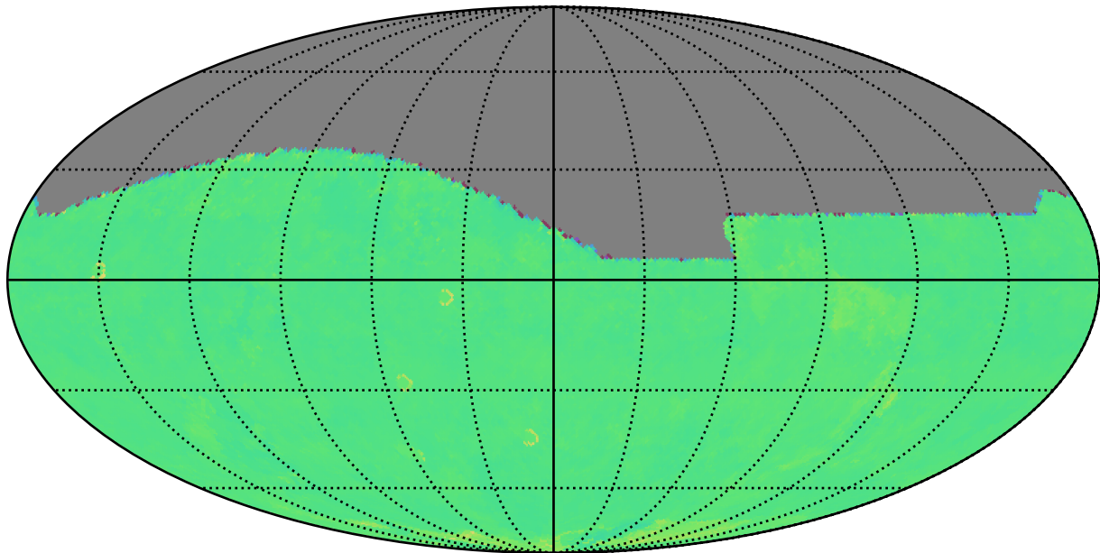
too_elab_heavy_r64_d3_ugrizy_v3.4_10yrs r: Kuiper rotTelPos
