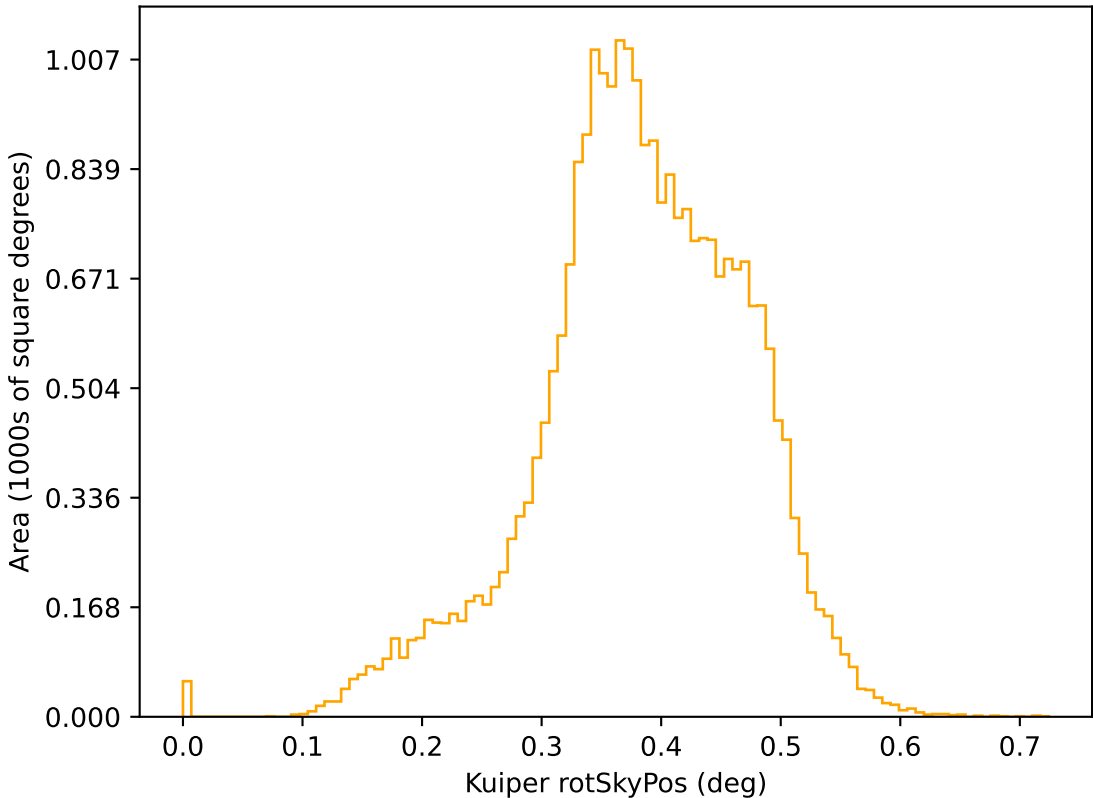
too_elab_heavy_r64_d3_ugrizy_v3.4_10yrs r: Kuiper rotSkyPos
