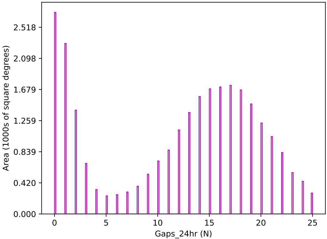
too_elab_heavy_r64_d3_ugrizy_v3.4_10yrs z band: Gaps_24hr
