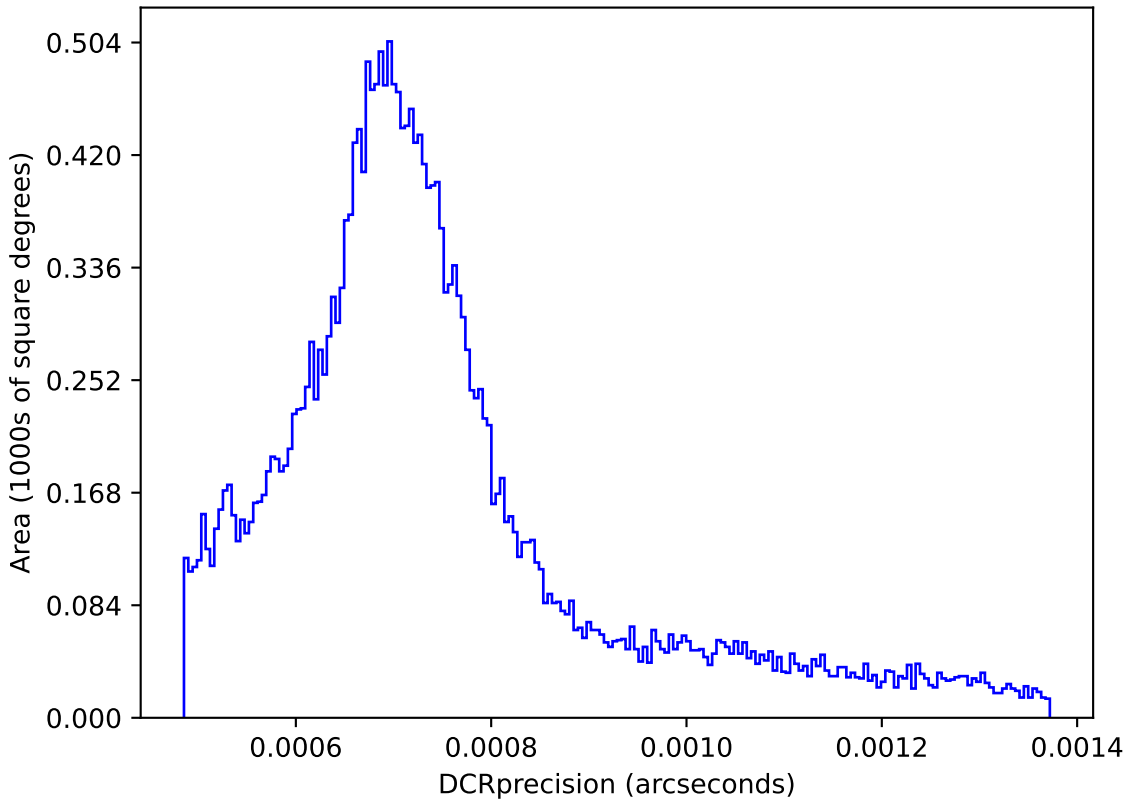
too_elab_heavy_r64_d3_ugrizy_v3.4_10yrs : DCRprecision
