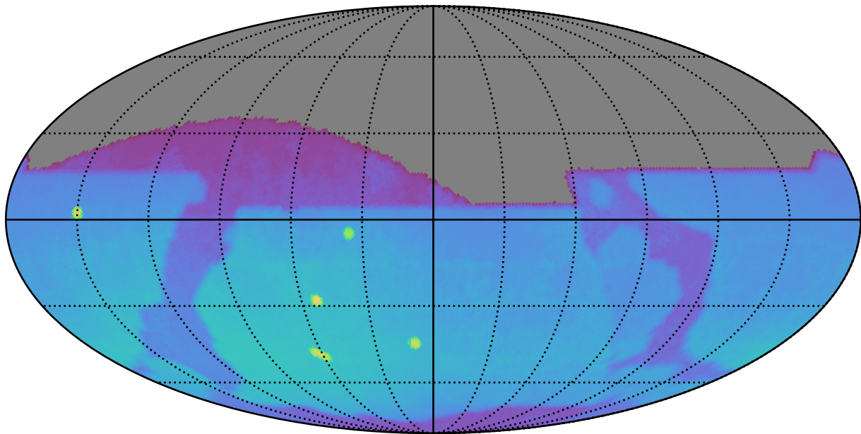
too_elab_heavy_r64_d3_ugrizy_v3.4_10yrs : Brown Dwarf, L7
