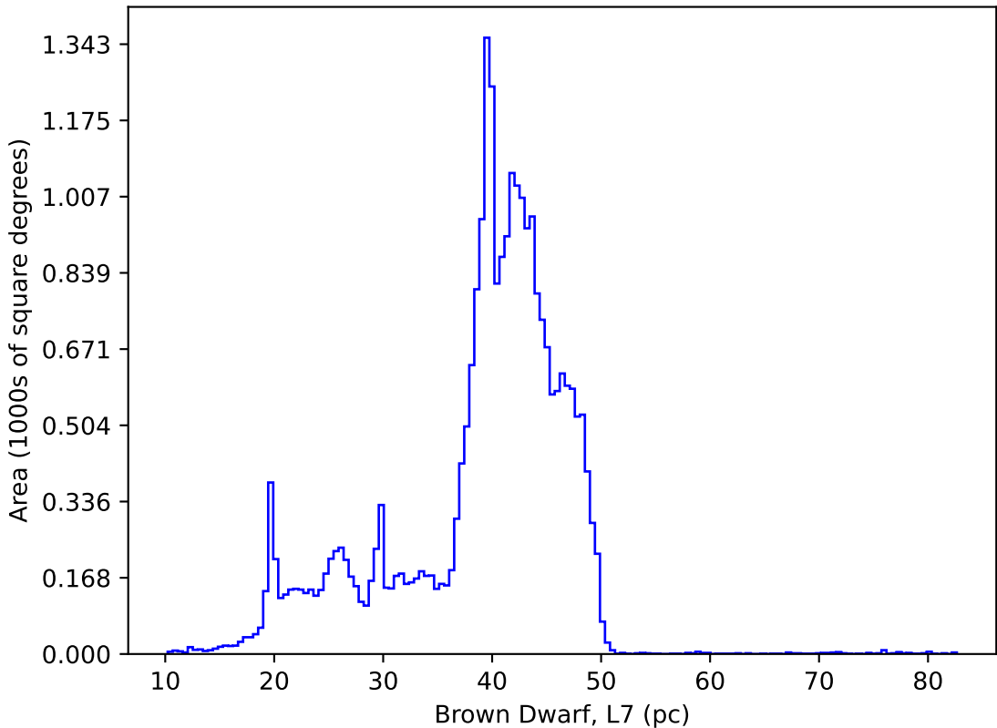
too_elab_heavy_r64_d3_ugrizy_v3.4_10yrs : Brown Dwarf, L7
