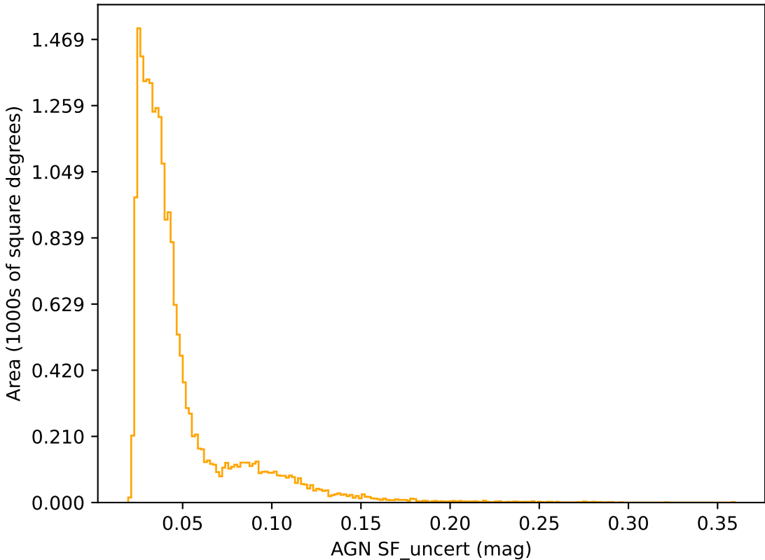
too_elab_heavy_r64_d3_ugrizy_v3.4_10yrs r band: AGN SF_uncert
