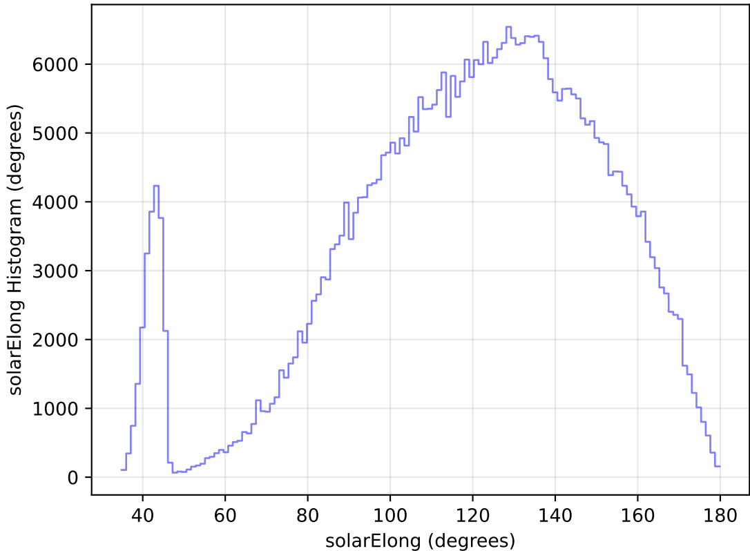
too_elab_heavy_r64_d3_ugrizy_v3.4_10yrs WFD z band: solarElong Histogram
