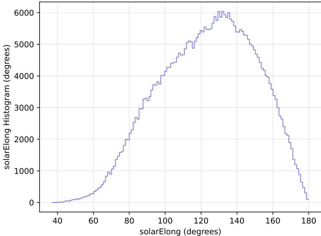
too_elab_heavy_r64_d3_ugrizy_v3.4_10yrs WFD y band: solarElong Histogram
