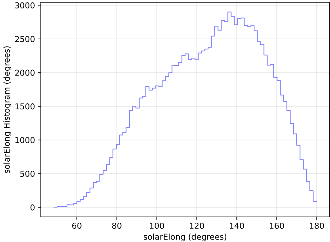
too_elab_heavy_r64_d3_ugrizy_v3.4_10yrs WFD u band: solarElong Histogram
