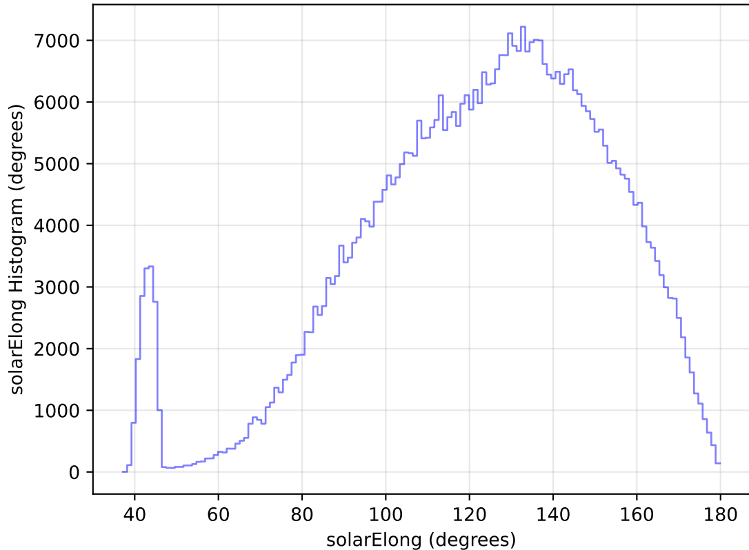
too_elab_heavy_r64_d3_ugrizy_v3.4_10yrs WFD r band: solarElong Histogram
