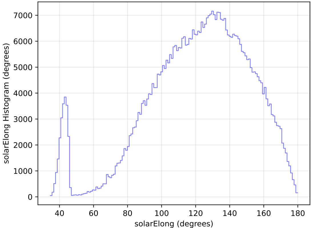
too_elab_heavy_r64_d3_ugrizy_v3.4_10yrs WFD i band: solarElong Histogram
