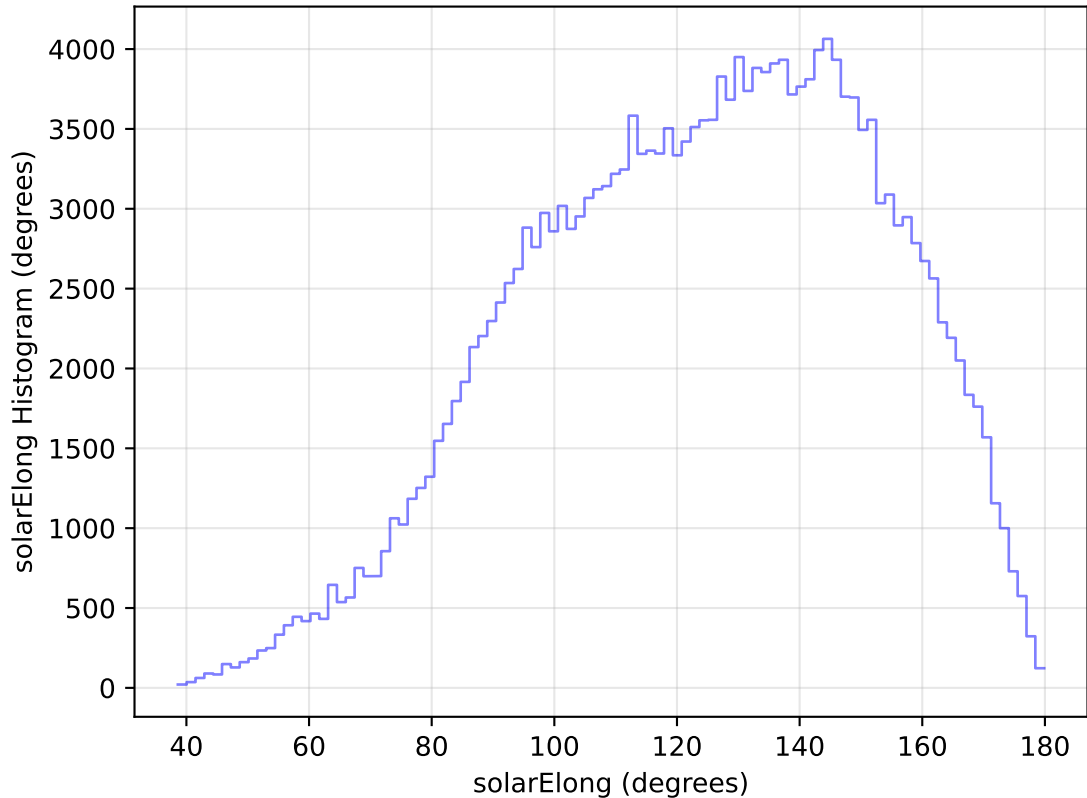
too_elab_heavy_r64_d3_ugrizy_v3.4_10yrs WFD g band: solarElong Histogram
