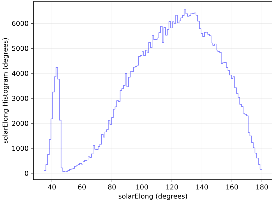
too_elab_heavy_r64_d3_ugrizy_v3.4_10yrs All sky z band: solarElong Histogram
