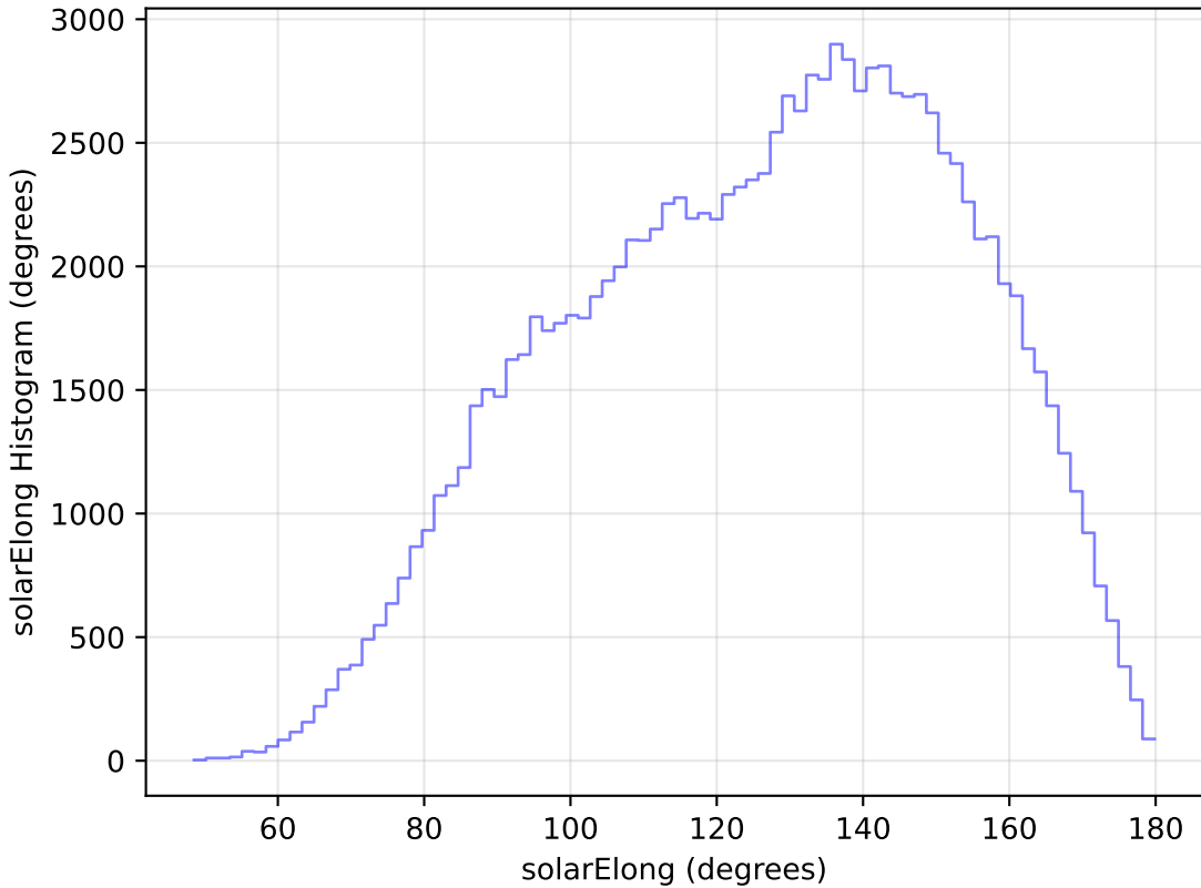
too_elab_heavy_r64_d3_ugrizy_v3.4_10yrs All sky u band: solarElong Histogram
