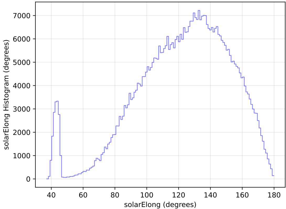
too_elab_heavy_r64_d3_ugrizy_v3.4_10yrs All sky r band: solarElong Histogram
