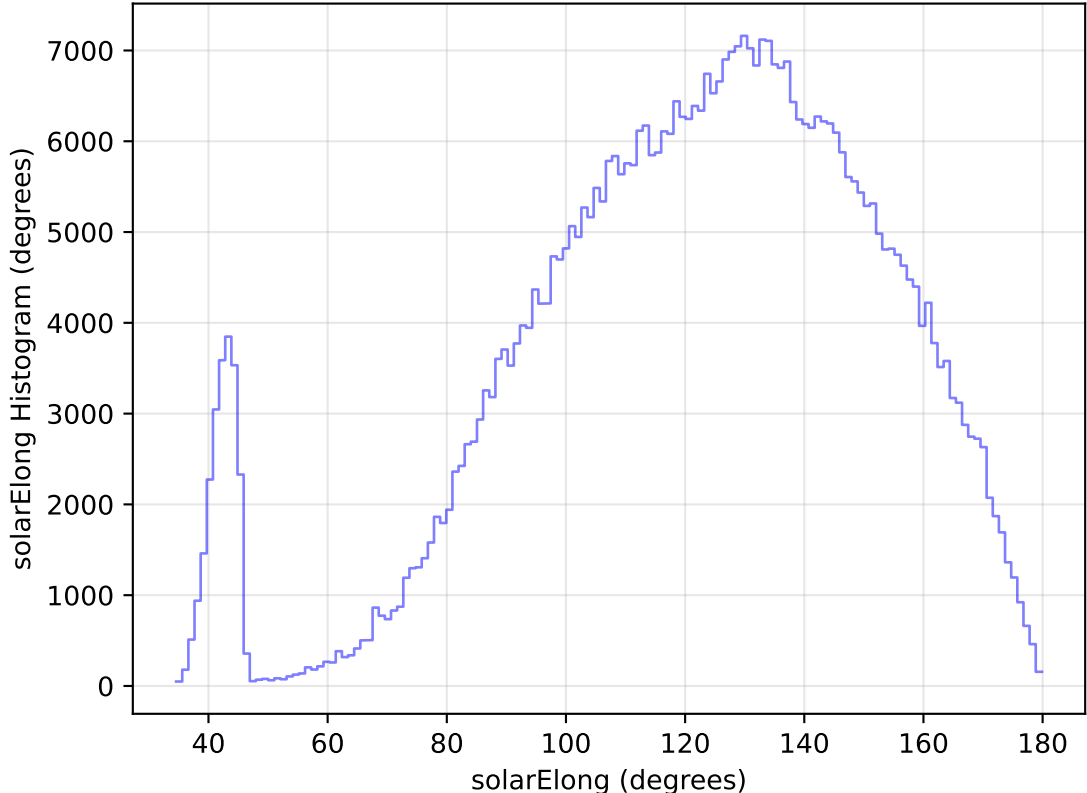
too_elab_heavy_r64_d3_ugrizy_v3.4_10yrs All sky i band: solarElong Histogram
