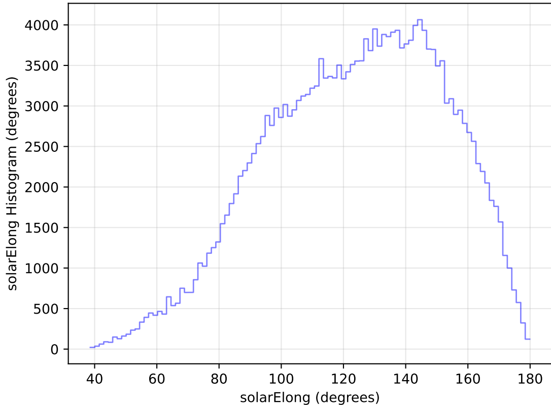
too_elab_heavy_r64_d3_ugrizy_v3.4_10yrs All sky g band: solarElong Histogram
