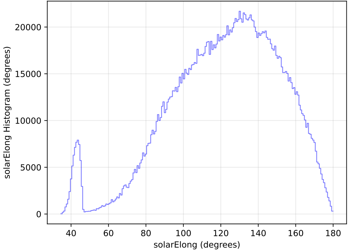
too_elab_heavy_r64_d3_ugrizy_v3.4_10yrs All sky all bands: solarElong Histogram
