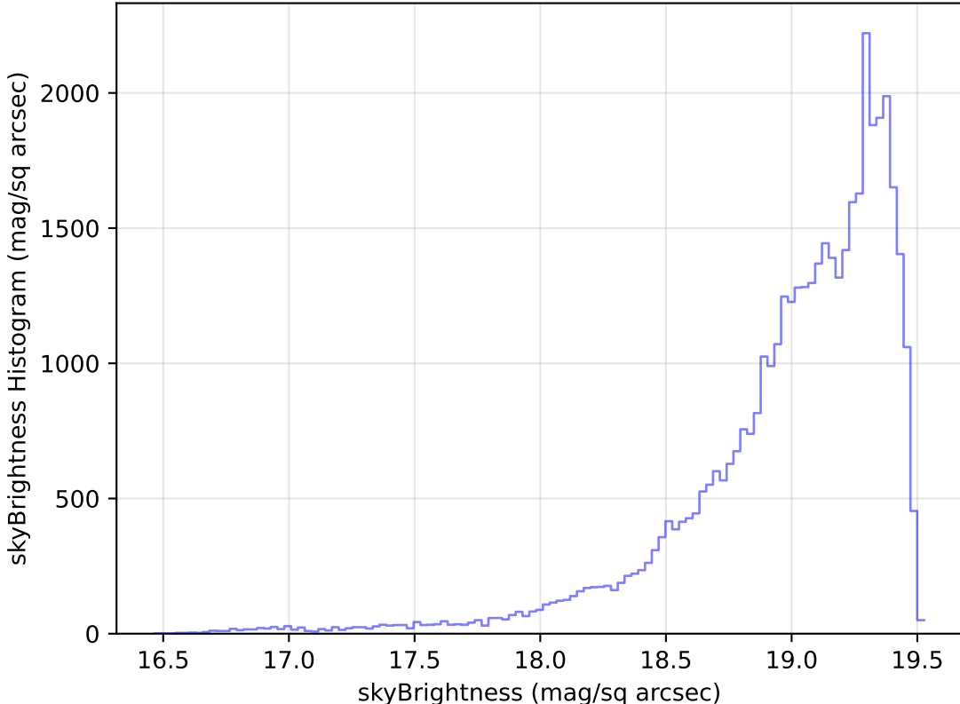
too_elab_heavy_r64_d3_ugrizy_v3.4_10yrs Yr 1 z band: skyBrightness Histogram
