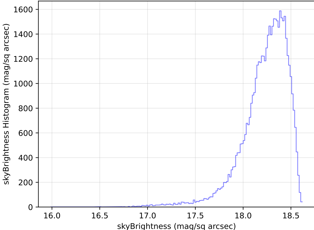
too_elab_heavy_r64_d3_ugrizy_v3.4_10yrs Yr 1 y band: skyBrightness Histogram
