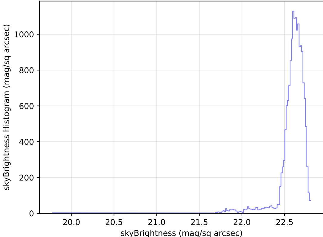
too_elab_heavy_r64_d3_ugrizy_v3.4_10yrs Yr 1 u band: skyBrightness Histogram
