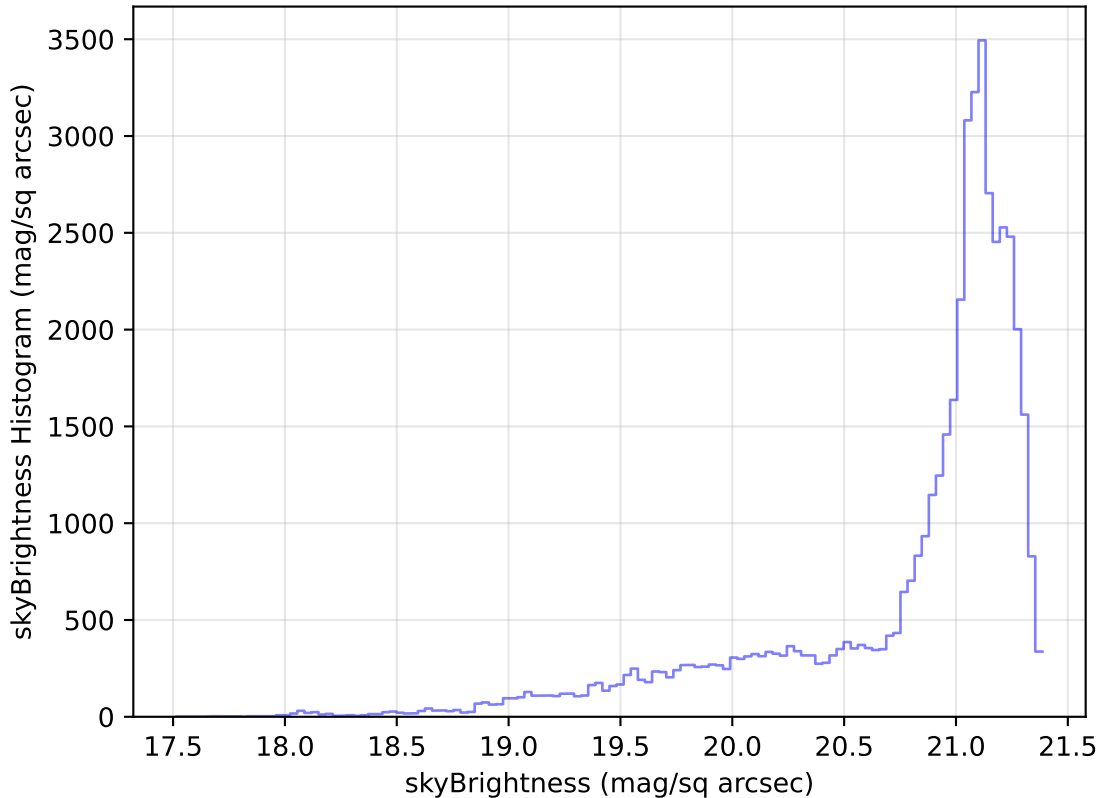
too_elab_heavy_r64_d3_ugrizy_v3.4_10yrs Yr 1 r band: skyBrightness Histogram
