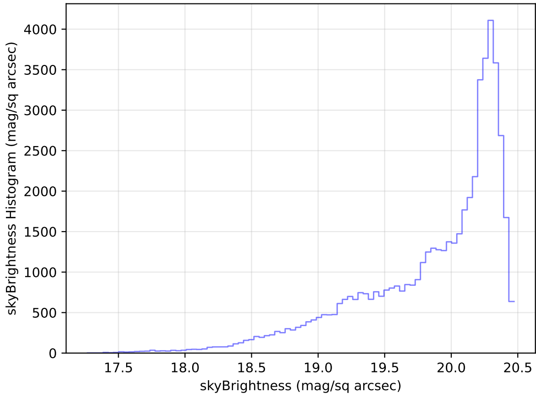
too_elab_heavy_r64_d3_ugrizy_v3.4_10yrs Yr 1 i band: skyBrightness Histogram
