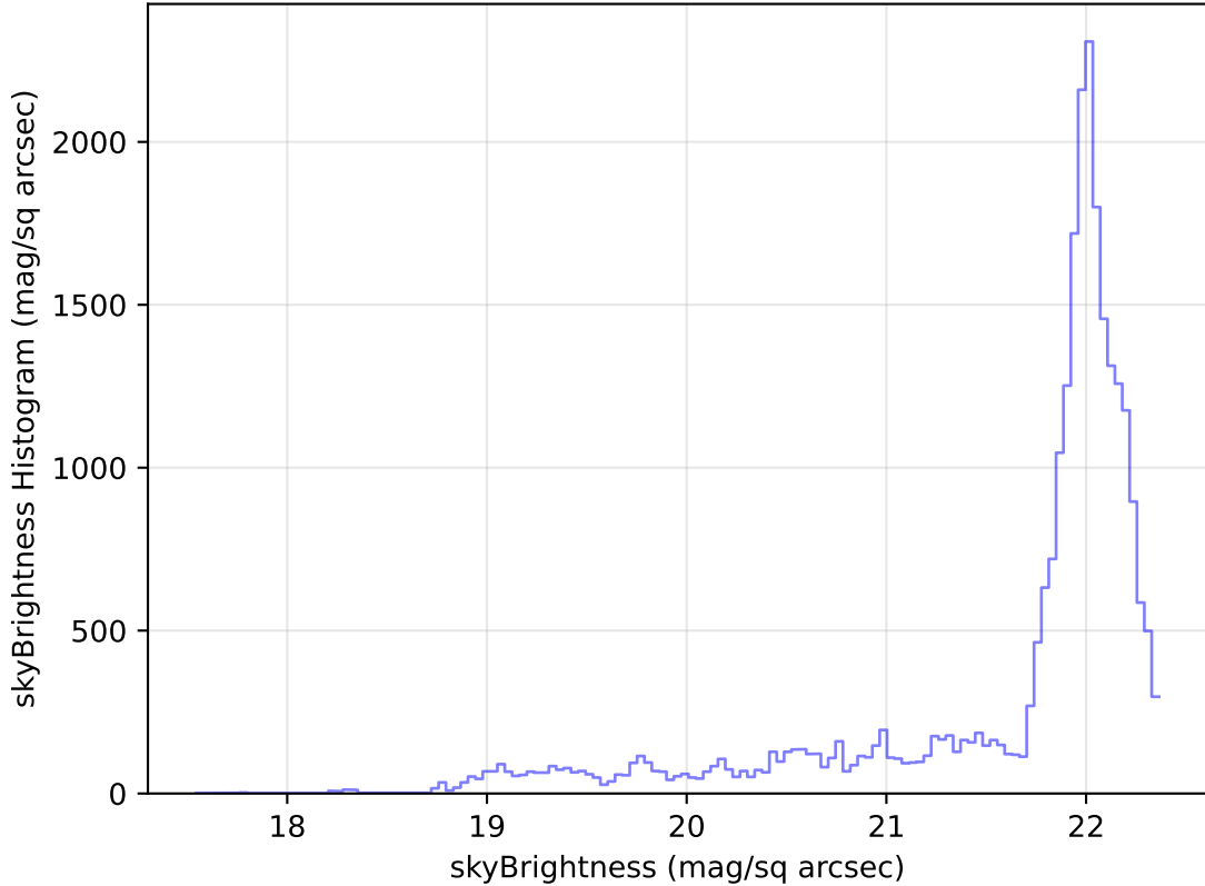
too_elab_heavy_r64_d3_ugrizy_v3.4_10yrs Yr 1 g band: skyBrightness Histogram
