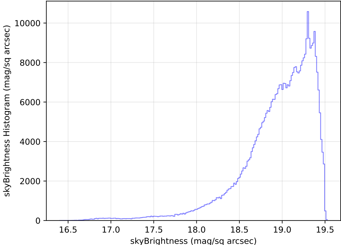
too_elab_heavy_r64_d3_ugrizy_v3.4_10yrs WFD z band: skyBrightness Histogram
