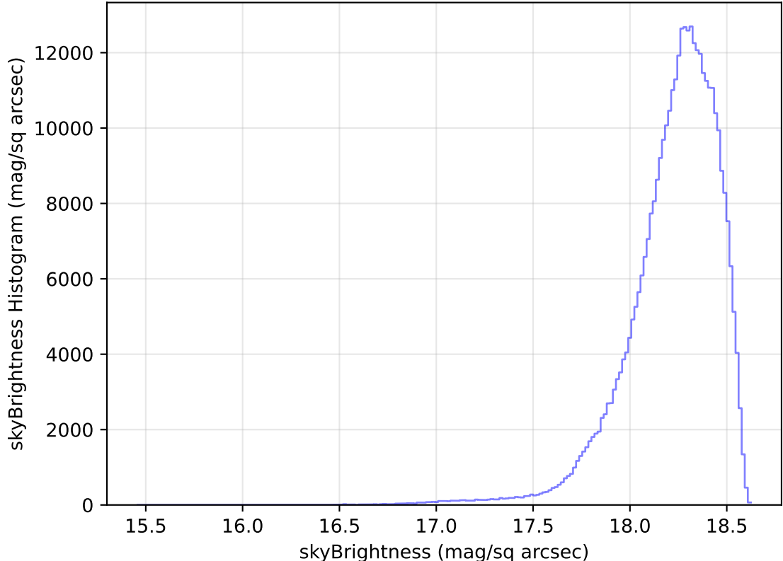
too_elab_heavy_r64_d3_ugrizy_v3.4_10yrs WFD y band: skyBrightness Histogram
