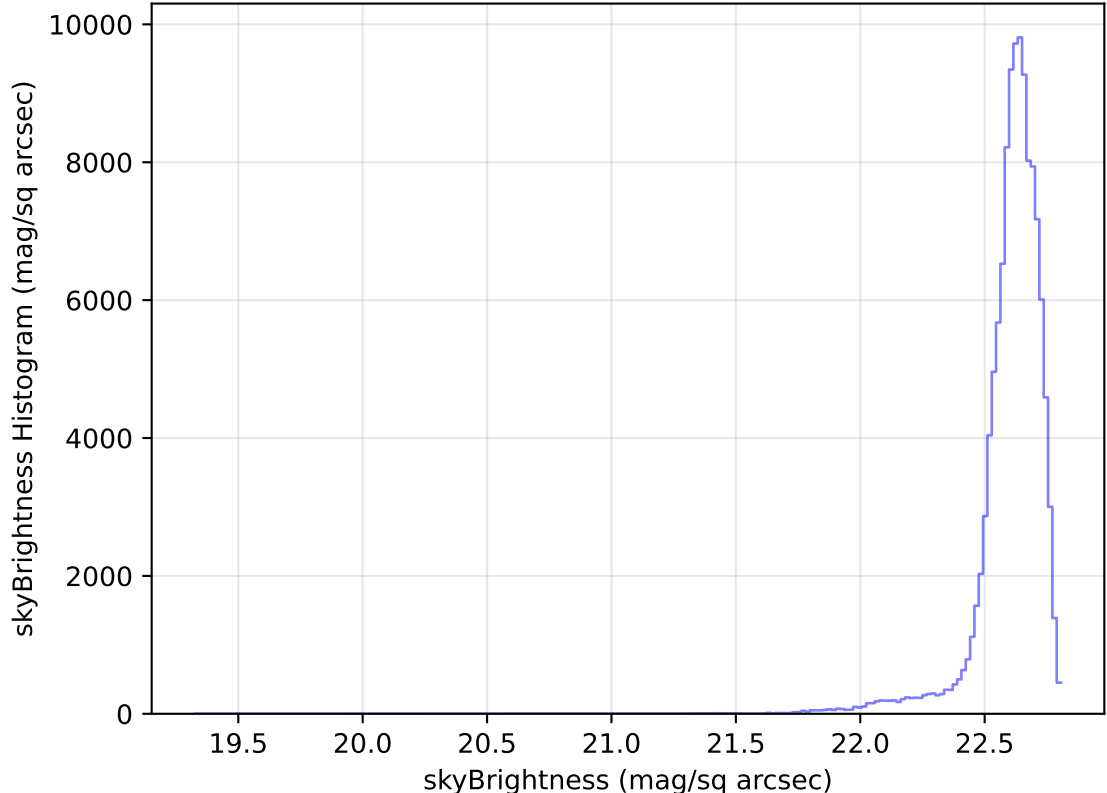
too_elab_heavy_r64_d3_ugrizy_v3.4_10yrs WFD u band: skyBrightness Histogram
