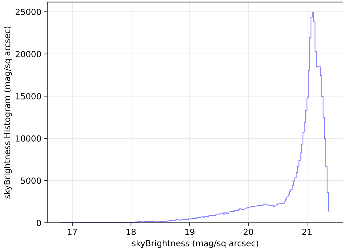
too_elab_heavy_r64_d3_ugrizy_v3.4_10yrs_WFD_r_band: skyBrightness Histogram
