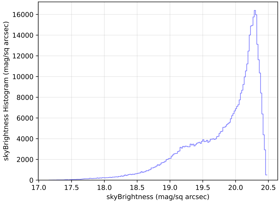
too_elab_heavy_r64_d3_ugrizy_v3.4_10yrs WFD i band: skyBrightness Histogram
