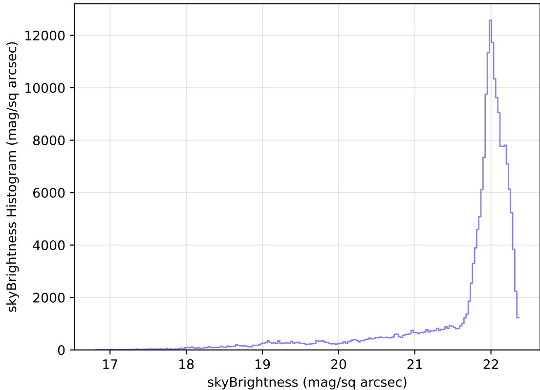
too_elab_heavy_r64_d3_ugrizy_v3.4_10yrs WFD g band: skyBrightness Histogram
