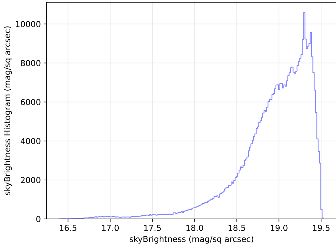
too_elab_heavy_r64_d3_ugrizy_v3.4_10yrs All sky z band: skyBrightness Histogram
