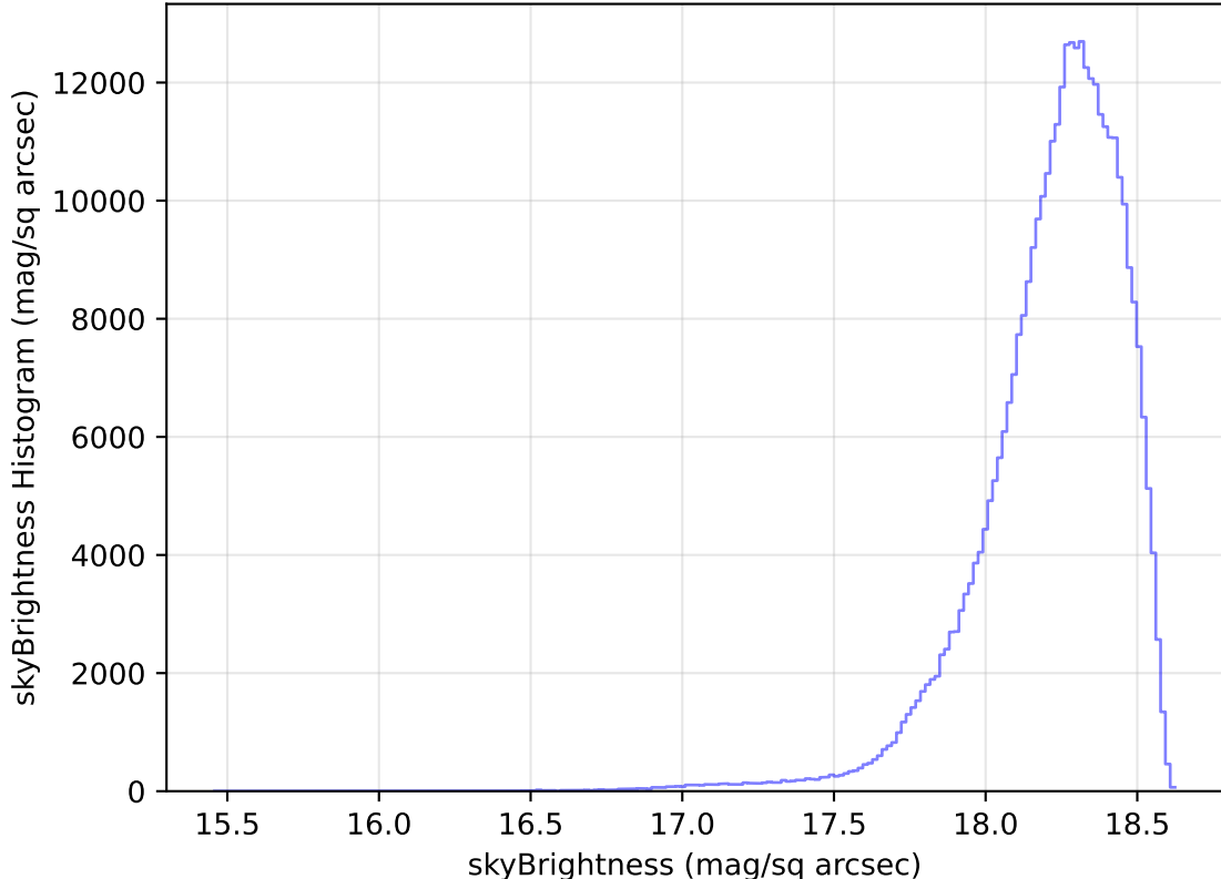
too_elab_heavy_r64_d3_ugrizy_v3.4_10yrs All sky y band: skyBrightness Histogram
