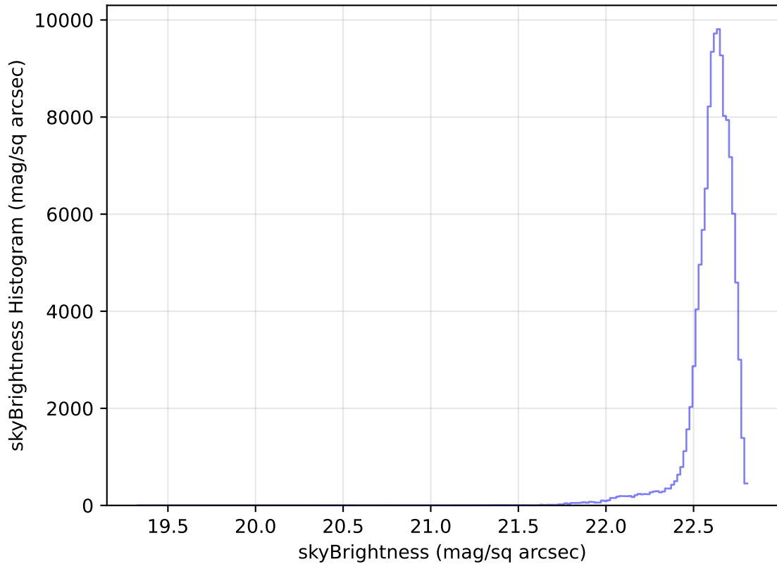
too_elab_heavy_r64_d3_ugrizy_v3.4_10yrs All sky u band: skyBrightness Histogram
