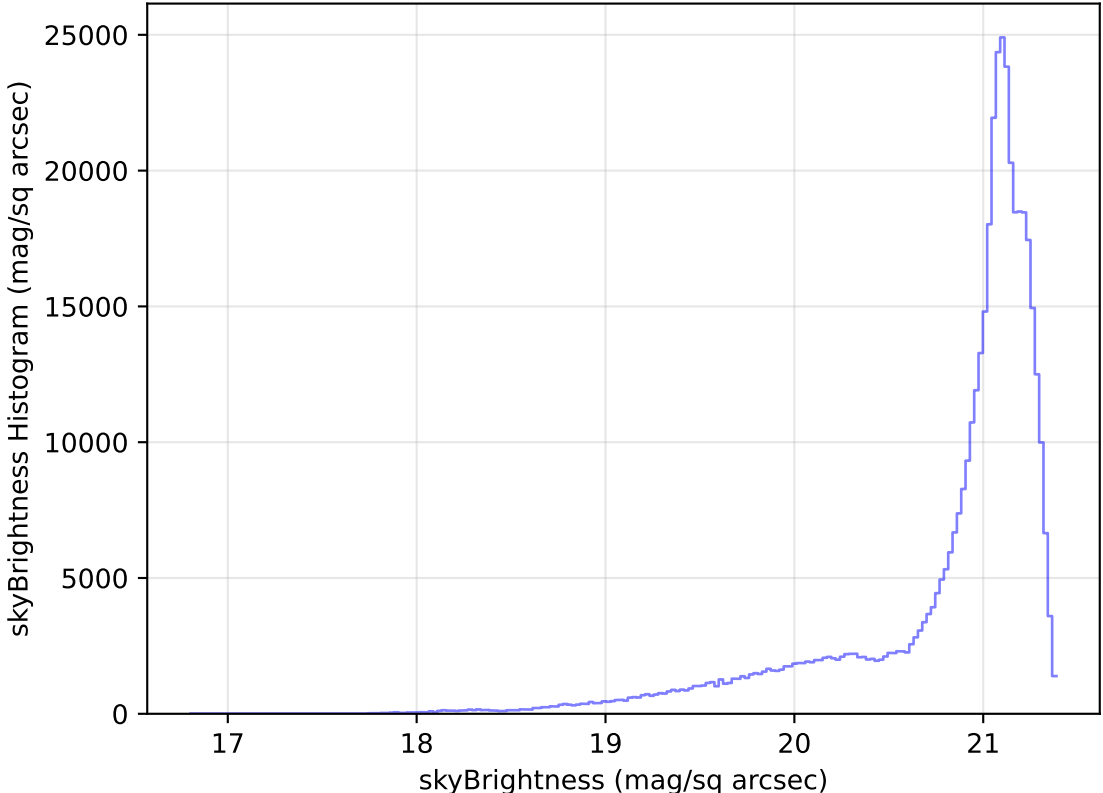
too_elab_heavy_r64_d3_ugrizy_v3.4_10yrs All sky r band: skyBrightness Histogram
