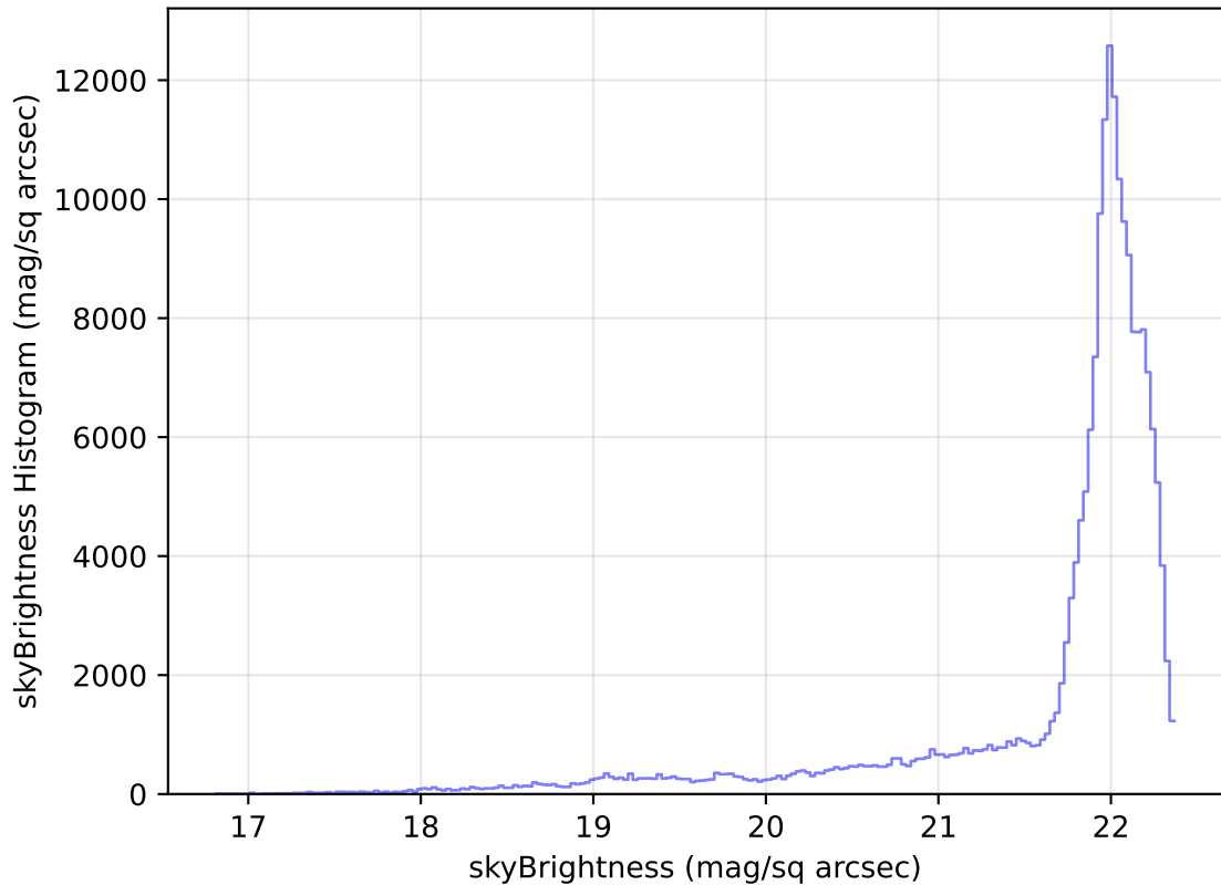
too_elab_heavy_r64_d3_ugrizy_v3.4_10yrs All sky g band: skyBrightness Histogram
