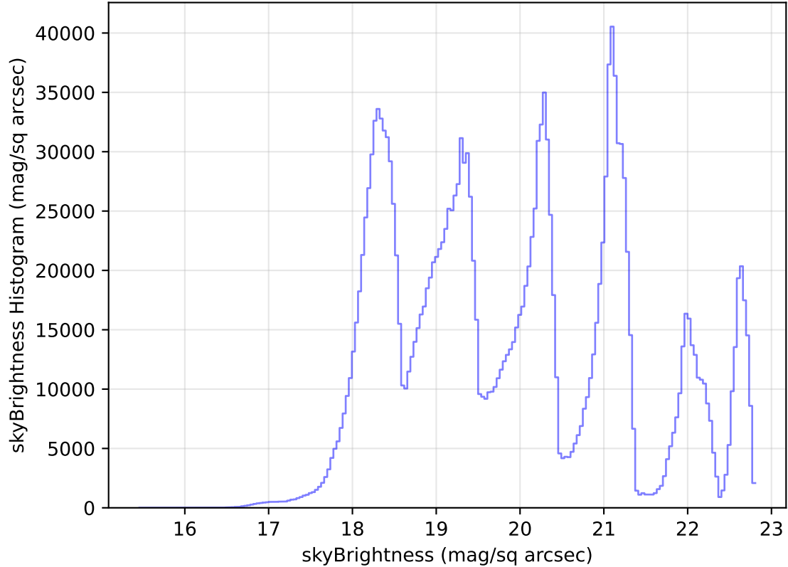
too_elab_heavy_r64_d3_ugrizy_v3.4_10yrs All sky all bands: skyBrightness Histogram
