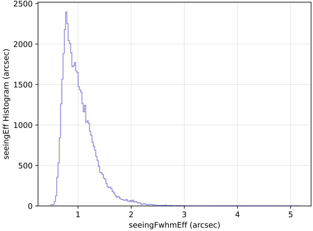
too_elab_heavy_r64_d3_ugrizy_v3.4_10yrs Yr 1 r band: seeingEff Histogram
