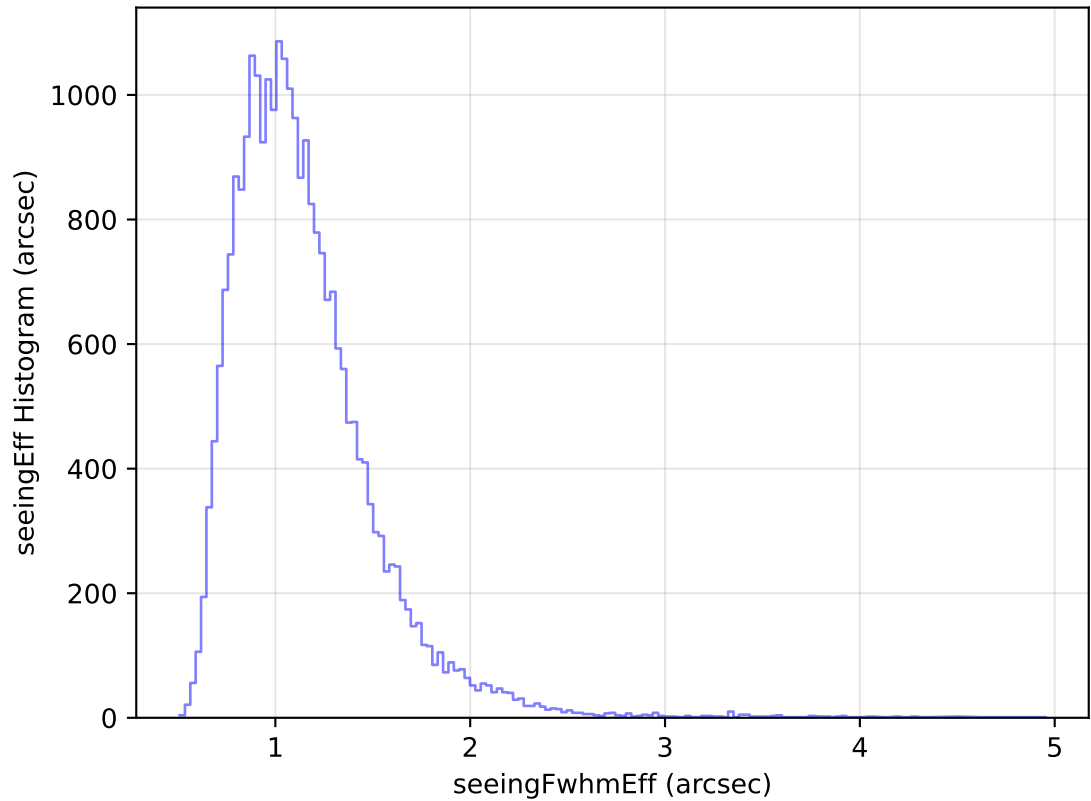
too_elab_heavy_r64_d3_ugrizy_v3.4_10yrs Yr 1 g band: seeingEff Histogram
