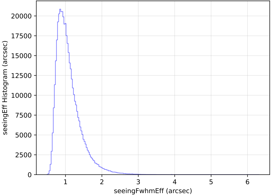
too_elab_heavy_r64_d3_ugrizy_v3.4_10yrs WFD z band: seeingEff Histogram
