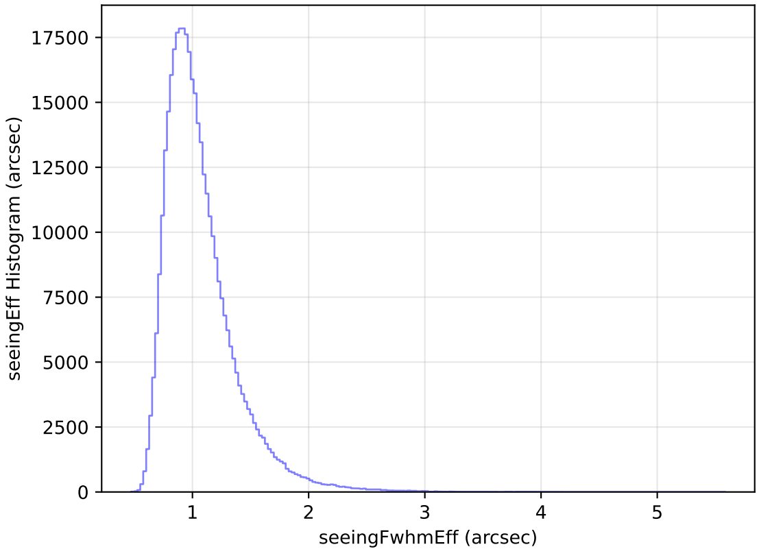
too_elab_heavy_r64_d3_ugrizy_v3.4_10yrs WFD y band: seeingEff Histogram
