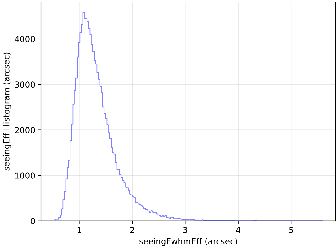
too_elab_heavy_r64_d3_ugrizy_v3.4_10yrs WFD u band: seeingEff Histogram
