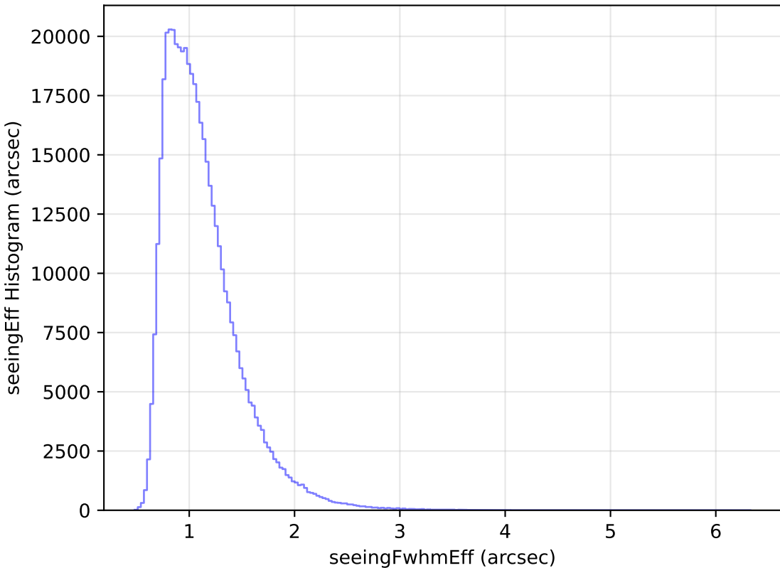
too_elab_heavy_r64_d3_ugrizy_v3.4_10yrs WFD r band: seeingEff Histogram
