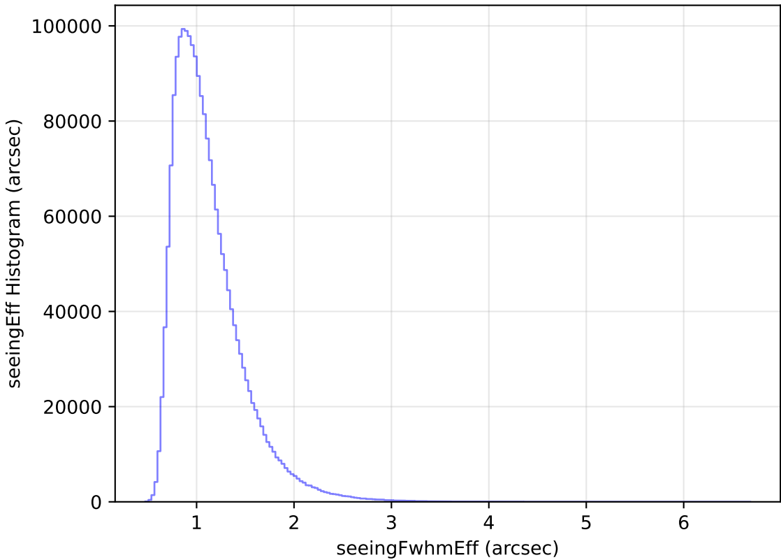
too_elab_heavy_r64_d3_ugrizy_v3.4_10yrs WFD all bands: seeingEff Histogram
