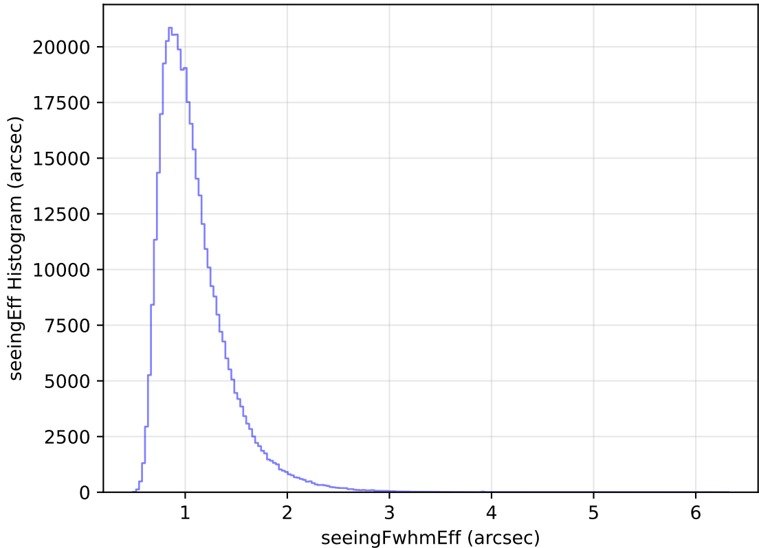
too_elab_heavy_r64_d3_ugrizy_v3.4_10yrs All sky z band: seeingEff Histogram
