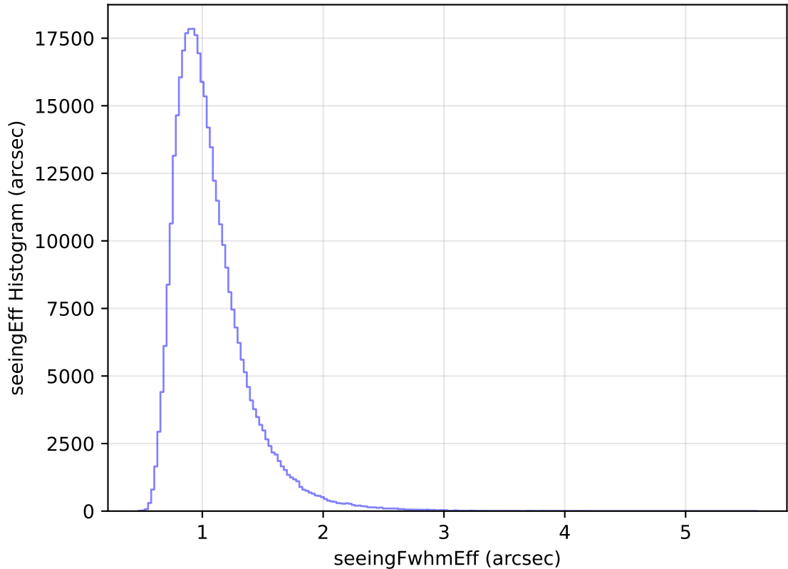
too_elab_heavy_r64_d3_ugrizy_v3.4_10yrs All sky y band: seeingEff Histogram
